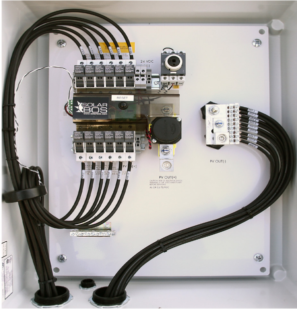
SolarBOS AFCI Combiner, 600 VDC, 200A contactor, 12 input circuits, NEMA-4X fiberglass enclosure
