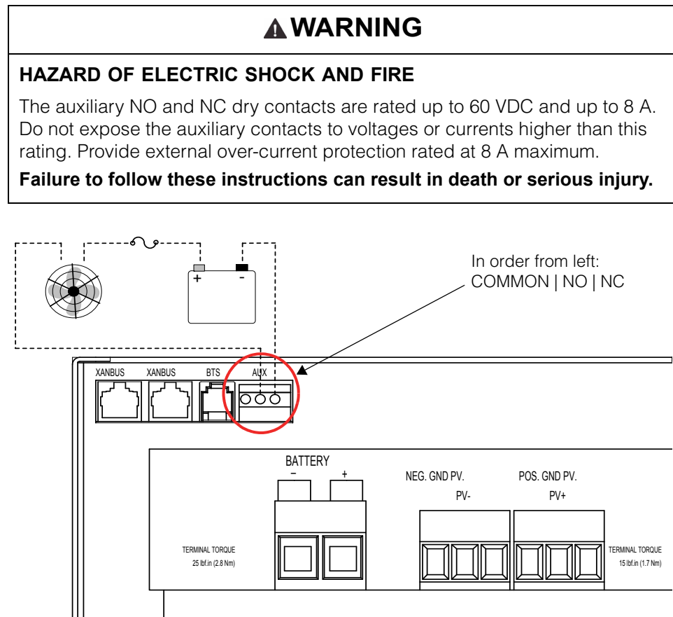
Figure 2-11 Auxiliary Output Vent Fan Application
