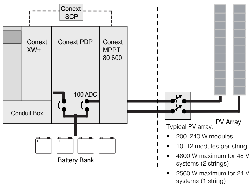
Figure 1-1 Typical Installation
