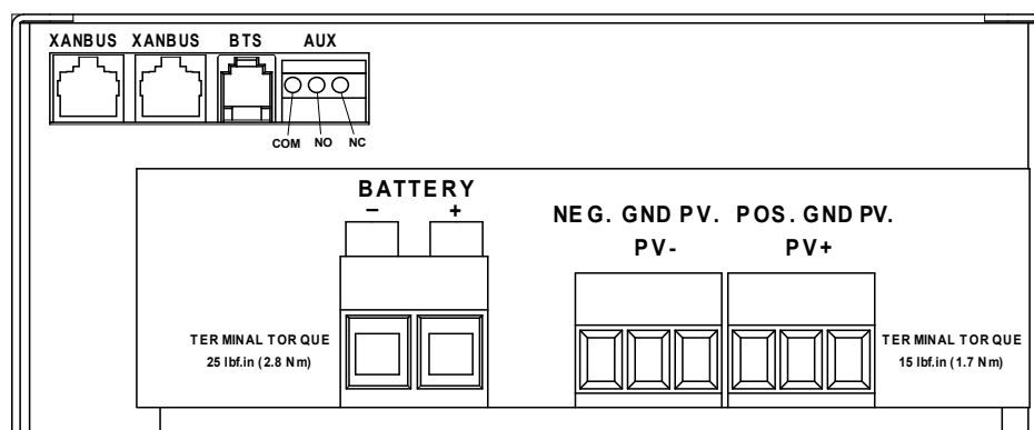
Figure 2-8 DC Terminal Connector Locations
