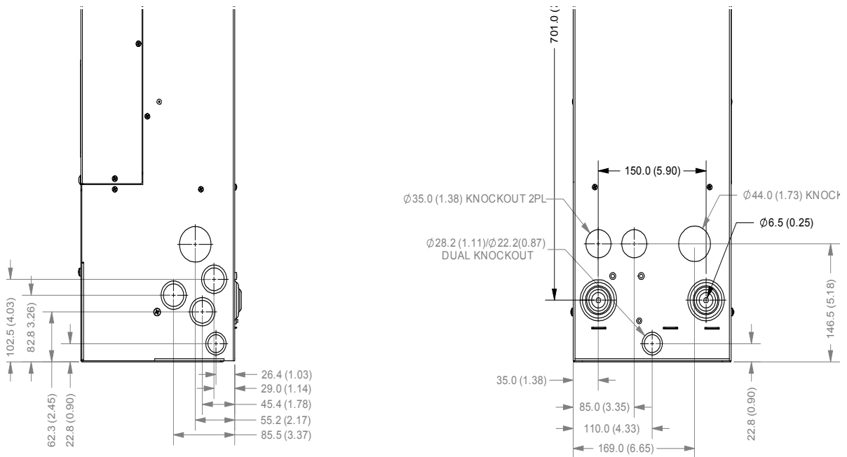
Figure 2-4 Knockout Dimensions
