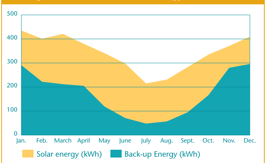
Example of Annual Solar Energy Contribution
