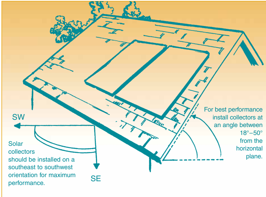
7 Solar collectors should be positioned facing southeast to southwest.
