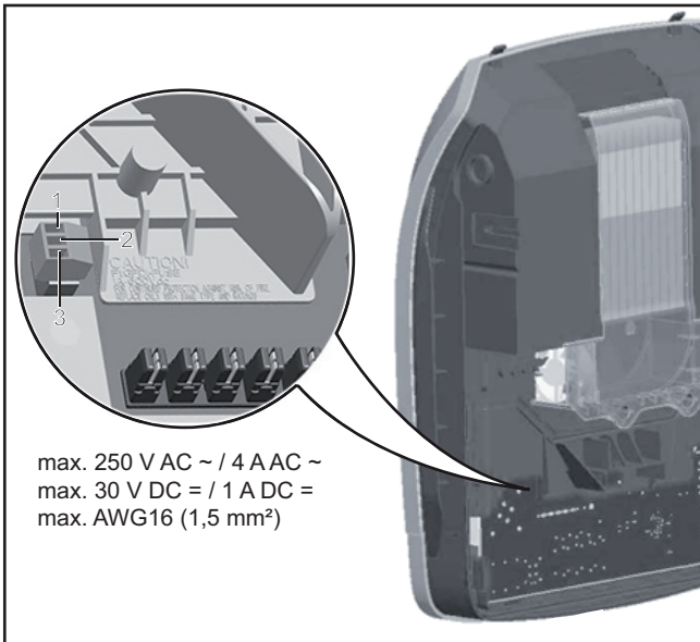
Floating switch contact with mating connector
