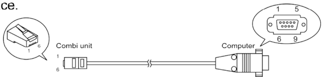
Figure 19. RS-232 cable
