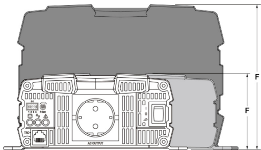
Figure 6. SP series drawing (AC output/Front View)
