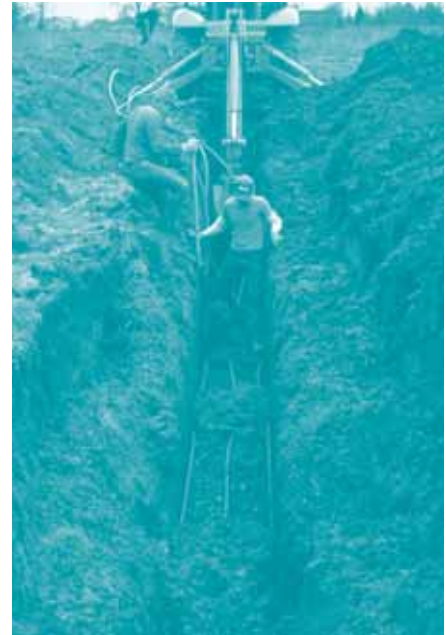
A backhoe is used to dig a horizontal trench for laying a ground loop.
