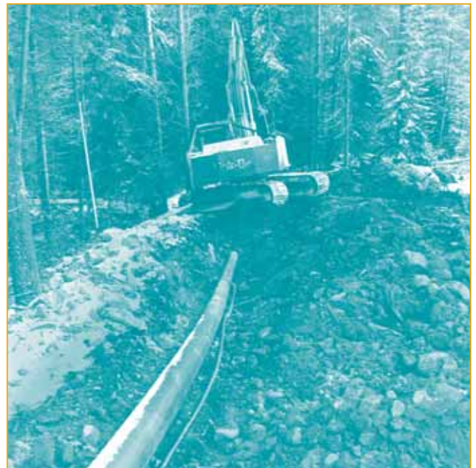
Figure 29. Burying a 20-cm (8-in.) Penstock pipe (photo courtesy of Thomson and Howe Energy Systems Inc.)
