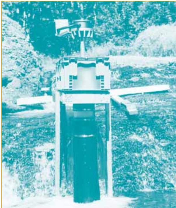
Figure 23. A 1-kW rated low-head battery-based system (photo courtesy of Energy Systems & Design)
